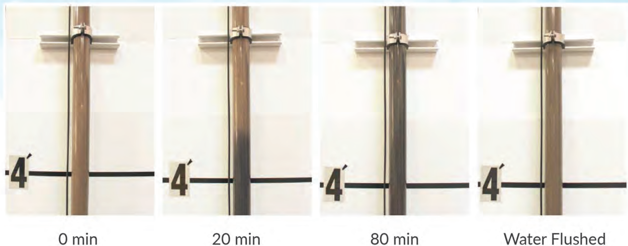
Figure 2. Visible PlumeStop migration front and coating residue following water-flush.
