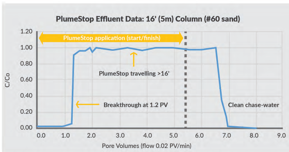
Figure 3. PlumeStop breakthrough dynamic - 16' (5m) column study.
