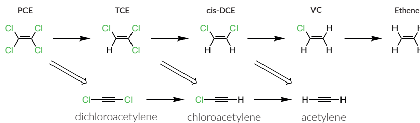
Figure 1: Chlorinated ethene degradation pathways and products. The top pathway with single line arrows represent the reductive dechlorination (hydrogenolysis) pathway. The lower pathway with downward facing double line arrows represent the beta- elimination pathway.
